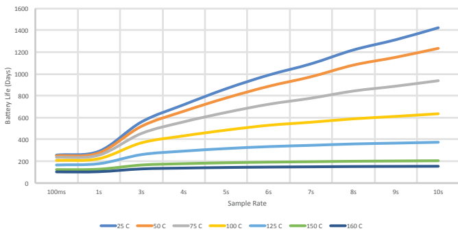
Gen 2 Quartz: PMX 150/165 1CC
